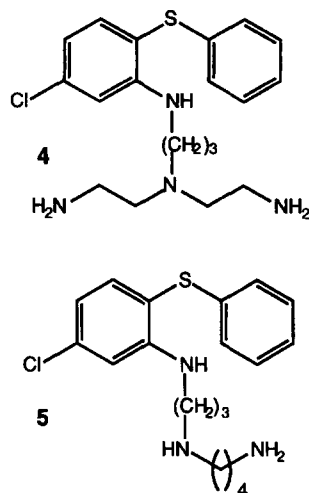
Figure 2. Structures of compounds 4 and 5.
