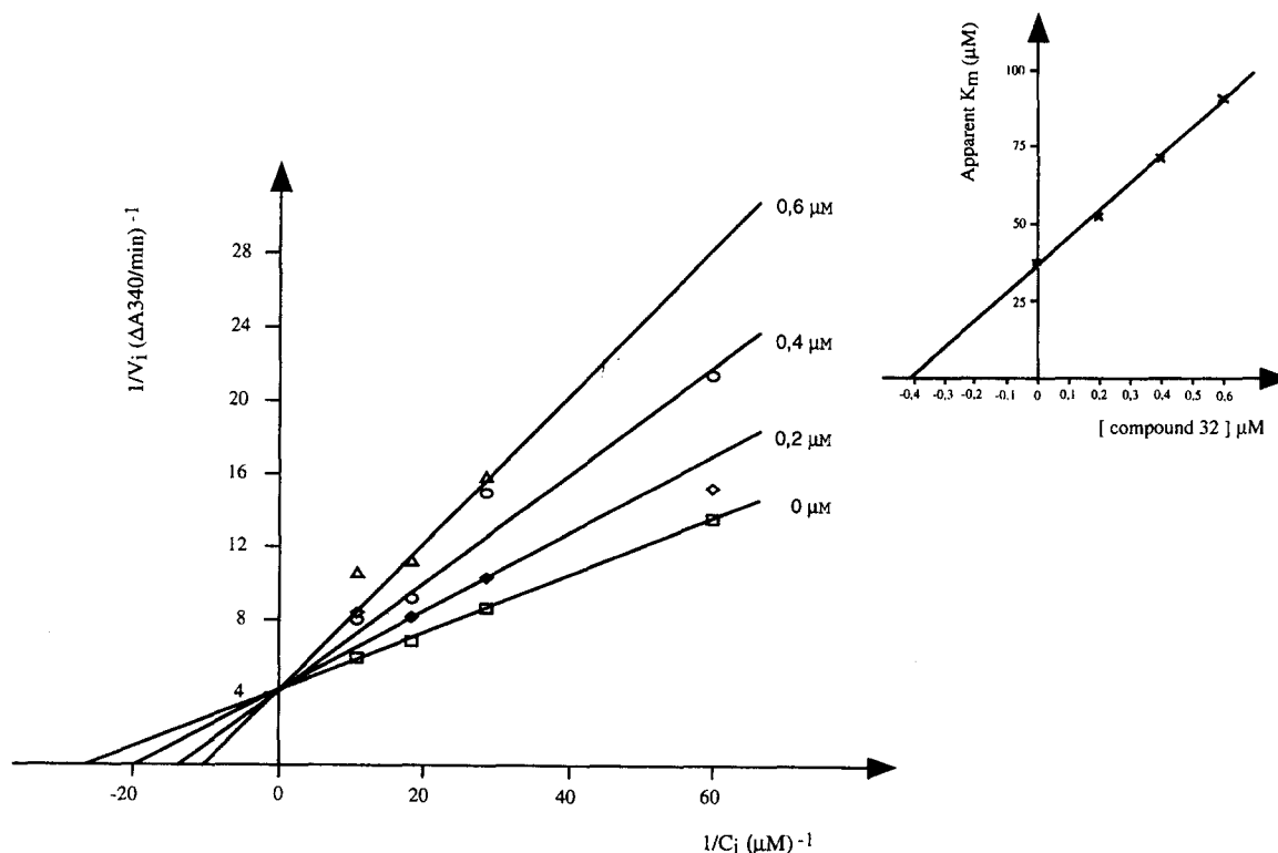
Figure 3. Competitive-type inhibition of TR by compound 32. Lineweaver–Burk plot of 1/v vs 1/[S] at different concentrations of 32 (0–0.6 \mu M) and the corresponding slope report of apparent K_m vs [I] .
