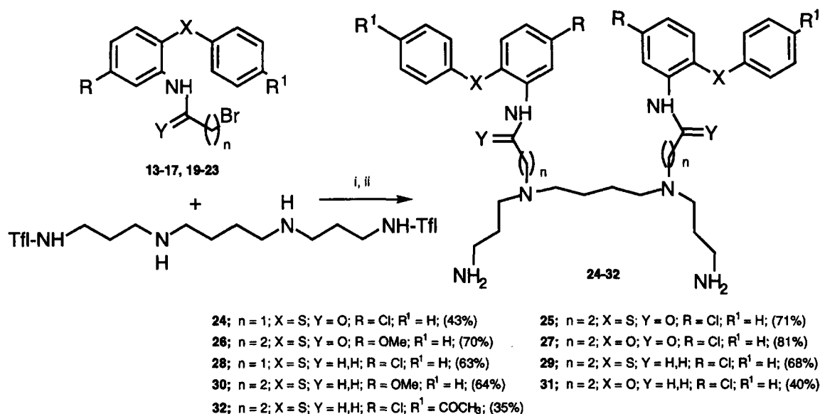
Scheme 2. Synthesis of spermine derivatives 24–32 . Reagents and conditions: (i) 6 equiv DiEA, CH_3CN , reflux, three days; (ii) for preparation of 24–27 : 5 equiv LiOH, H_2O , THF:H_2O (2:1), ultrasonics, 3 h, 25 °C; for preparation of 28–32 : 5 equiv LiOH, H_2O , THF:H_2O (2:1), reflux, 3 h.
