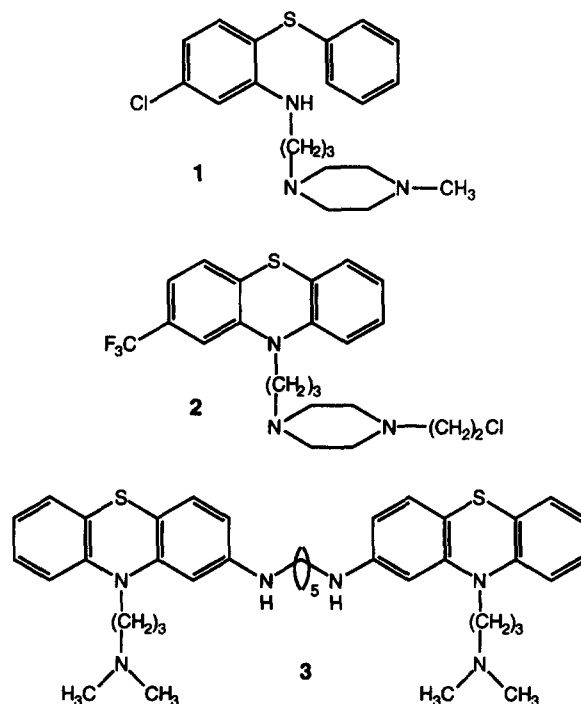
Figure 1. Structures of compounds 1 , 2 , and 3 .
