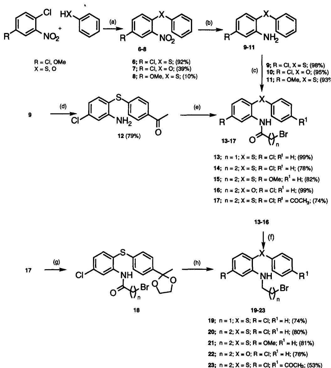
Scheme 1. Synthesis of bromodiphenyl compounds 13–23. Reagents and conditions: (a) for preparation of 6 and 7: \text{CH}_3\text{CO}_2\text{NH}_4 , abs EtOH, reflux, two days; for preparation of 8: KOH aq, reflux, 12 h; (b) Fe, concd HCl, 95% EtOH, reflux, 1 h; (c) for preparation of 13: 2-bromoacetyl bromide, ether, pyridine, 0 °C, 2 h; for preparation for 14–16: 3-bromopropionyl chloride, ether, pyridine, 0 °C, 2 h; (d) acetyl chloride, \text{AlCl}_3 , \text{CS}_2 , rt, 3 h; (e) 3-bromopropionyl chloride, ether, pyridine, 0 °C, 2 h; (f) \text{BH}_3/\text{THF} , THF, 0–25 °C, 4 h; (g) ethylene glycol, PTSA catal., toluene, reflux, 12 h; (h) \text{BH}_3/\text{THF} , THF, 0–25 °C, 4 h then HCl 4 N.
